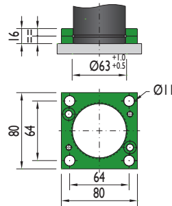
XCV-1500
